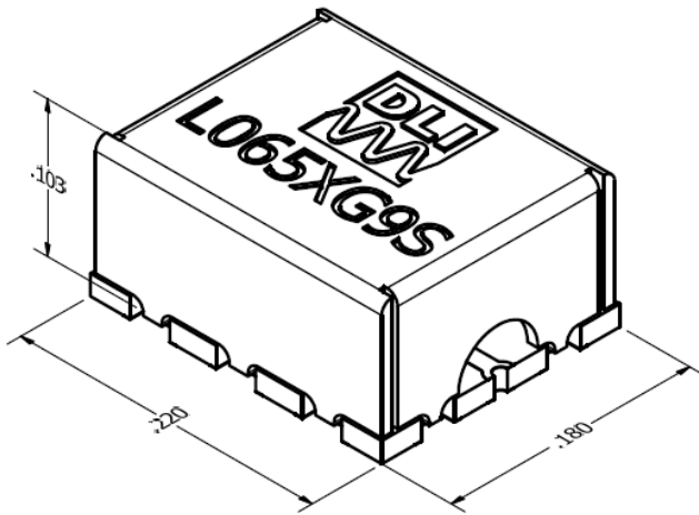
Isometric View
